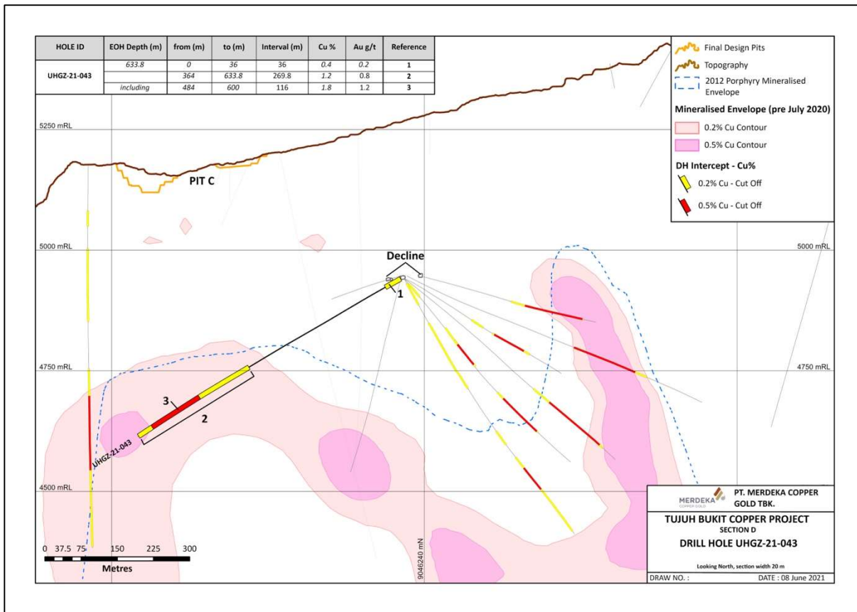
Figure 5: Drill section D, showing drill holes UHGZ-21-043 along with mineralised envelopes and drilling intercept information.
