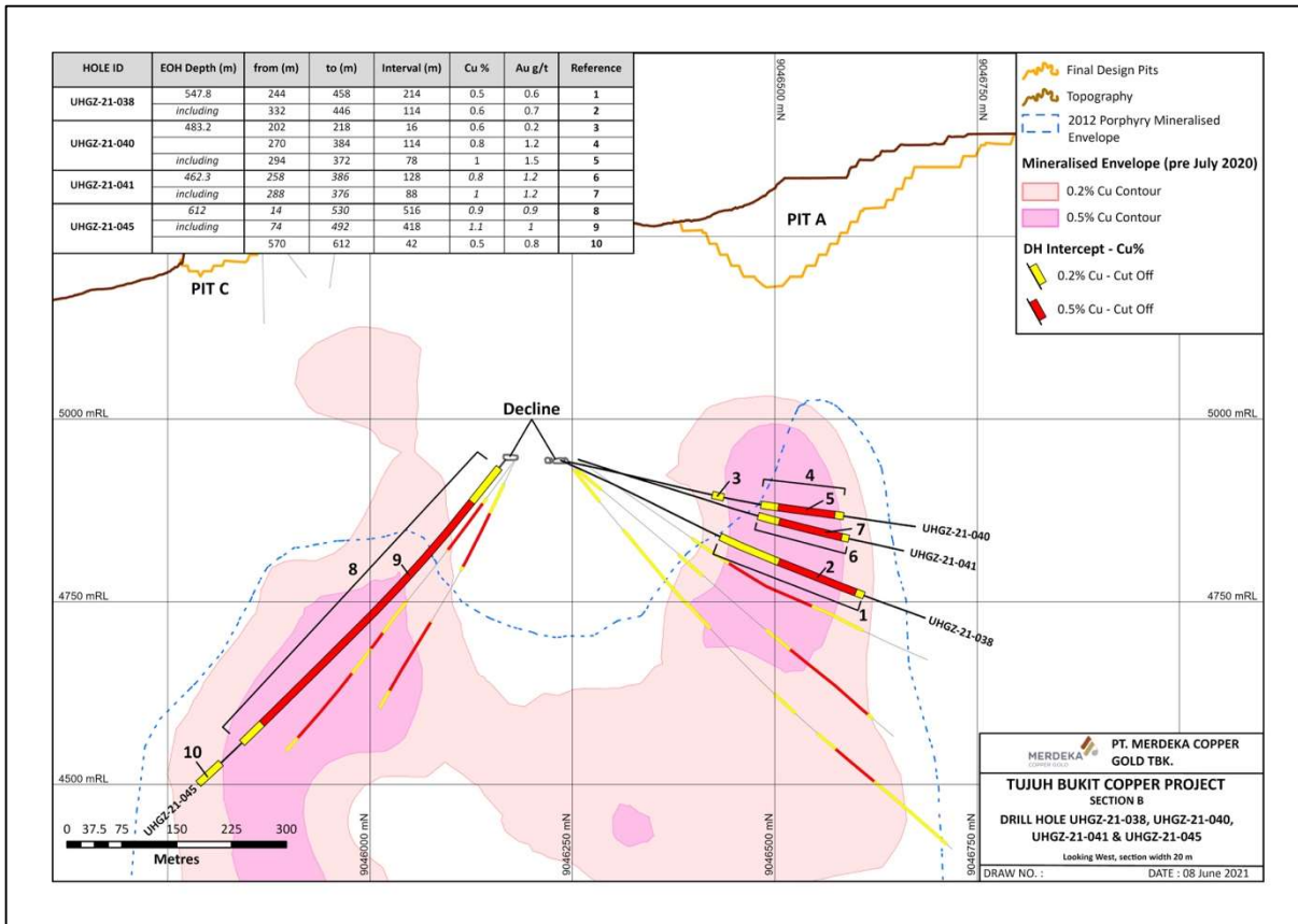
Figure 3: Drill section B, showing drill holes UHGZ-21-038, UHGZ-21-040, UHGZ-21-041 & UHGZ-21-045 along with mineralised envelopes and drilling intercept information.
