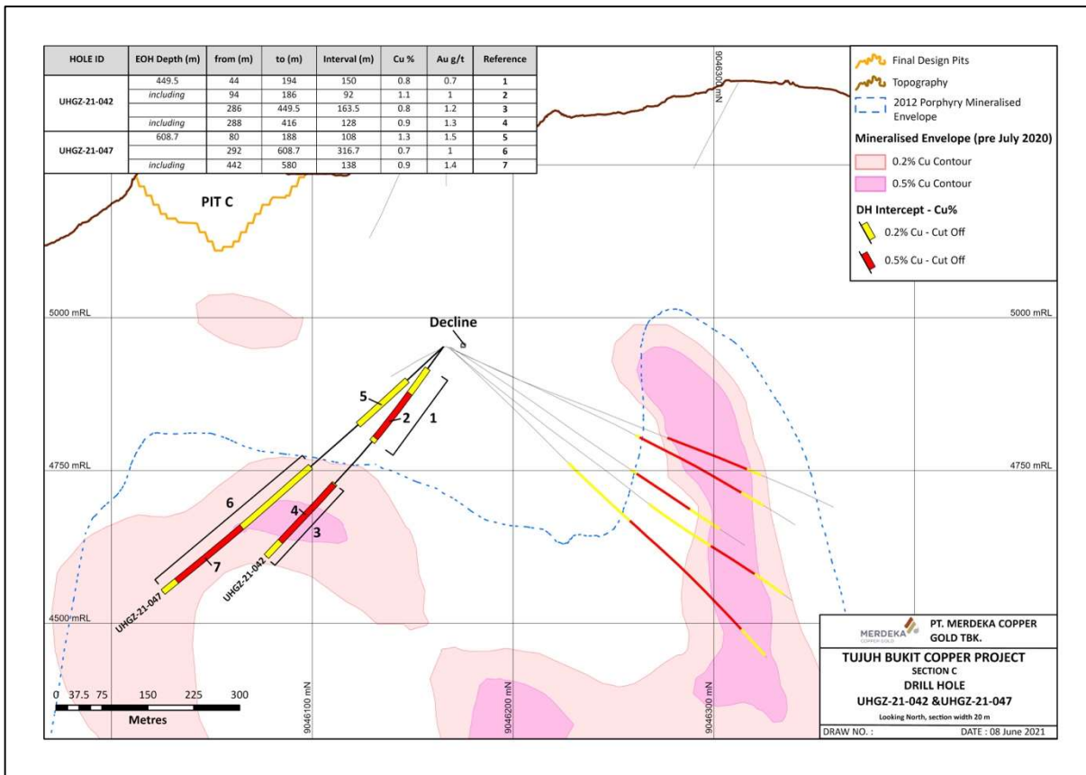
Figure 4: Drill section C, showing drill hole UHGZ-21-042 and UHGZ-21-047 along with mineralised envelopes and drilling intercept information.
