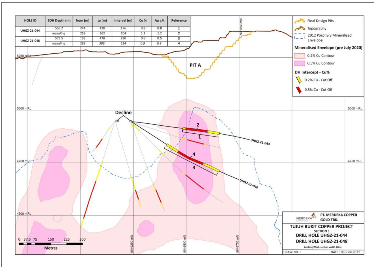
Figure 6: Drill section E, showing drill hole UHGZ-21-048 along with mineralised envelopes and drilling intercept information.
