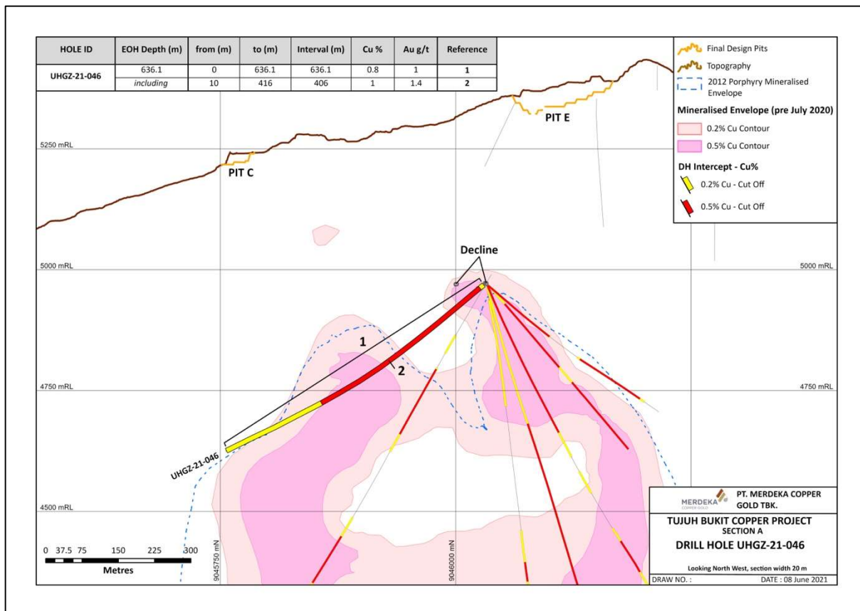
Figure 2: Drill section A, showing drill hole UHGZ-21-046 along with mineralised envelopes and drilling intercept information.
